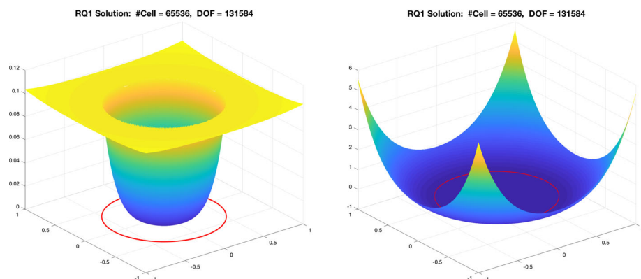
Fig. 4 IFE solutions for Example 5.1 with (\beta^-, \beta^+) = (1, 1000) and (\beta^-, \beta^+) = (1000, 1)
