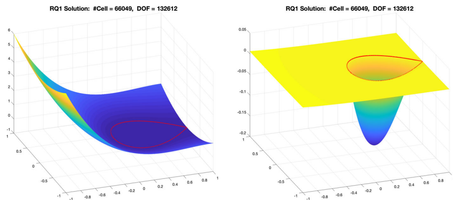
Fig. 5 IFE solutions for Example 5.2 with (\beta^-, \beta^+) = (1, 1000) and (\beta^-, \beta^+) = (1000, 1)
