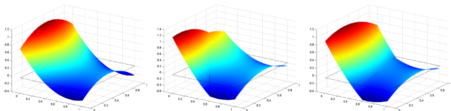
Fig. 3 Nonconforming FE/IFE local basis functions
