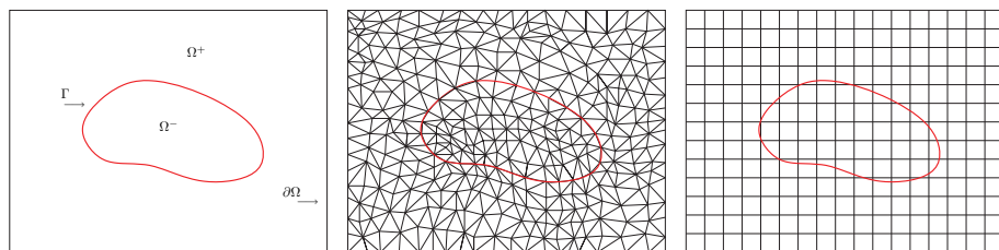
Fig. 1 Body-fitting mesh and non-body-fitting mesh of an interface problem
