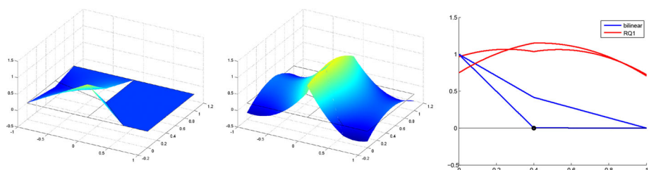
Fig. 7 Conforming Q_1 -IFE and nonconforming Q_1 -IFE bases with \beta^- = 1 , \beta^+ = 1000
