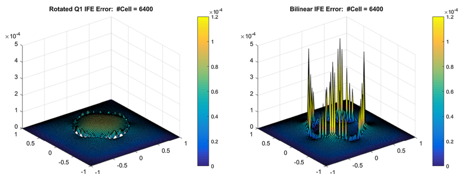
Fig. 6 Error surfaces of the nonconforming and conforming Q_1 -IFE solutions
