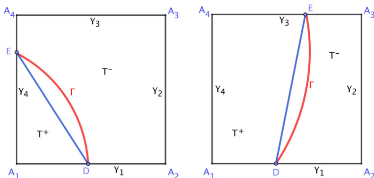
Fig. 2 Type I (left) and Type II (right) interface elements
