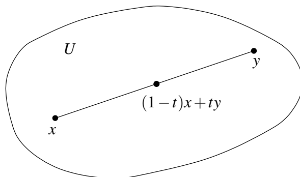
Figure 8.1: Convexity.
