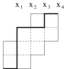
Figure 1: A lattice path \sigma with m(\sigma) = x_1^2 x_3 .
