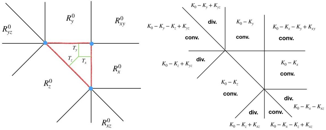
FIGURE 14. The regions R_{\sigma_1}^{\sigma_2} and their corresponding K_{\sigma_1, \sigma_2} functions
