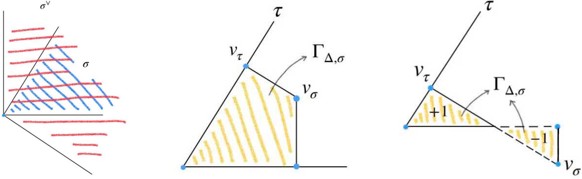
FIGURE 17. Two examples of the virtual polytopes \Gamma_{\Delta,\sigma} . In the first example the vertex v_\sigma lies in the cone \sigma and \Gamma_{\Delta,\sigma} is an actual polytope (a quadrangle). The convex chain \gamma_{\Delta,\sigma} is the characteristic function of the quadrangle. In the second example, v_\sigma lies outside \sigma and \Gamma_{\Delta,\sigma} is a virtual quadrangle. The convex chain \gamma_{\Delta,\sigma} is the function which has values 1 and -1 in the two shaded regions respectively.
