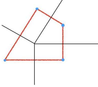
FIGURE 10. A usual quadrangle with its normal fan
