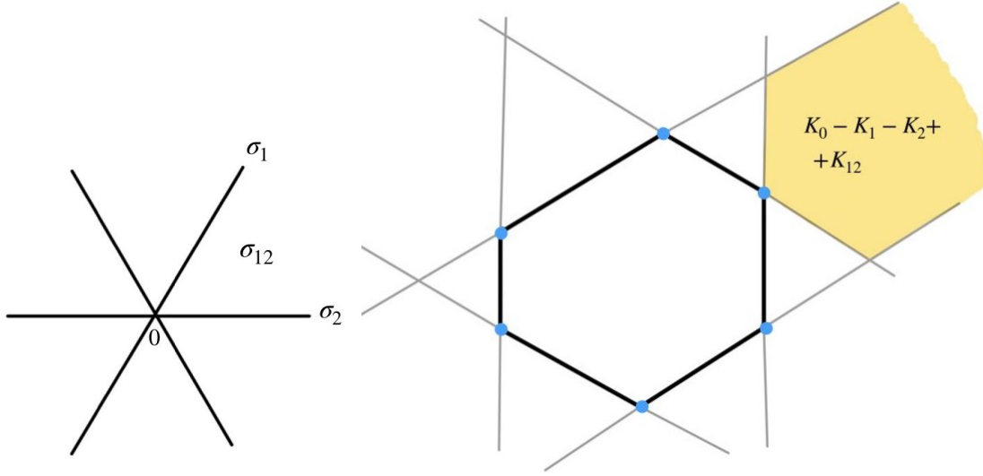
FIGURE 1. Left: a complete simplicial fan in V = \mathbb{R}^2 ; we have labeled three cones in the fan. Right: a polygon normal to the fan and regions obtained by drawing the outward face cones; the function k_\Delta in the shaded region is given by K_0 - K_1 - K_2 + K_{12} .
